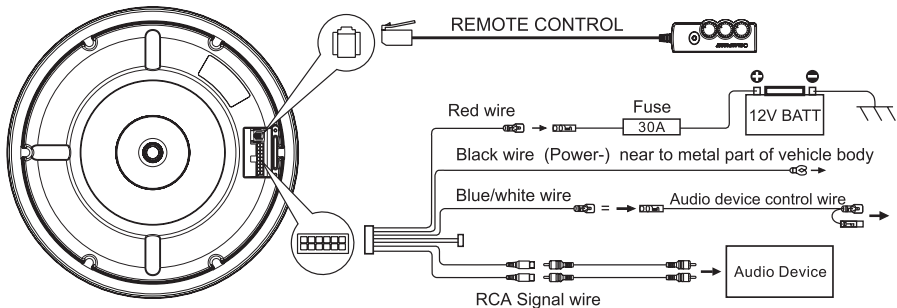
Diagram 2 (Low Level Input -Speaker Input)
