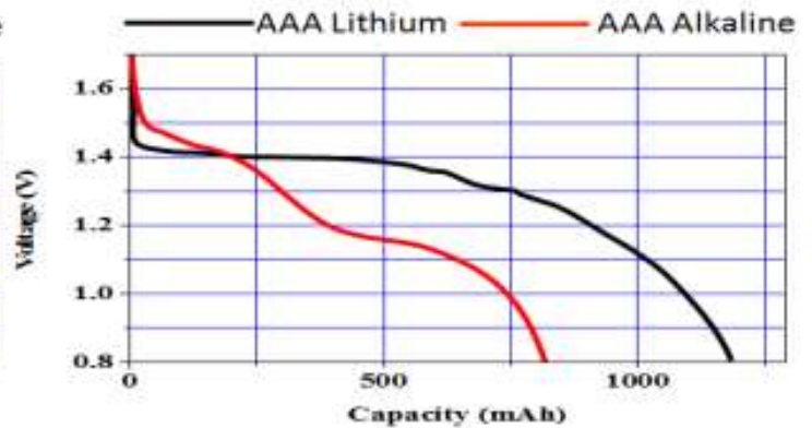
Constant current (50mA) discharge at 25°C
