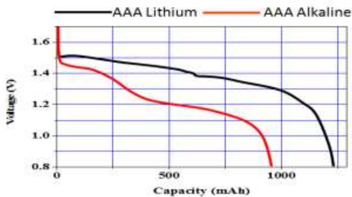
Constant current (50mA) discharge at 25°C
