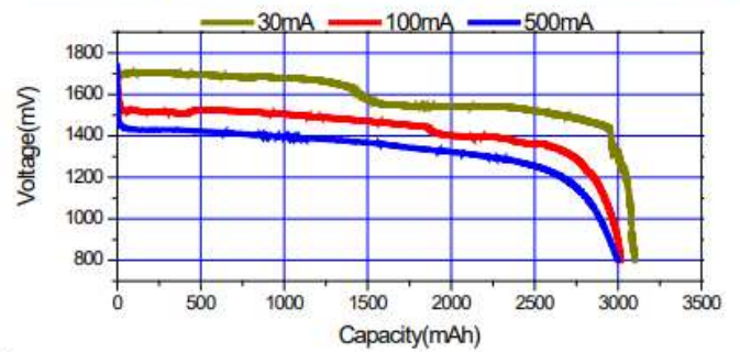
Discharge curve / Constant current discharge
