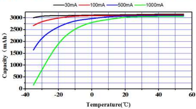
Temperature Effects on Capacity / Constant current discharge
