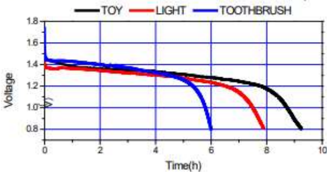
PORTABLE LIGHTING TOY 500mA 2min/13min 3.3ohm constant 3.9ohm 1hr/day
