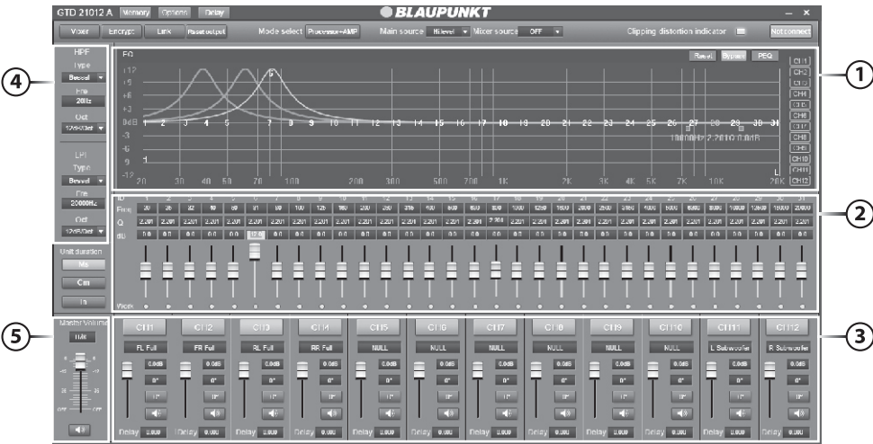
Channel Panel (31-band Tuning)
