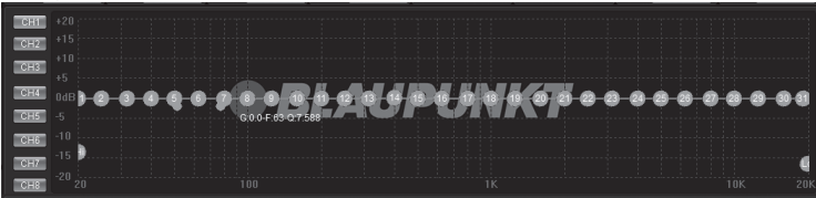
Channel Panel (31-band Tuning)
